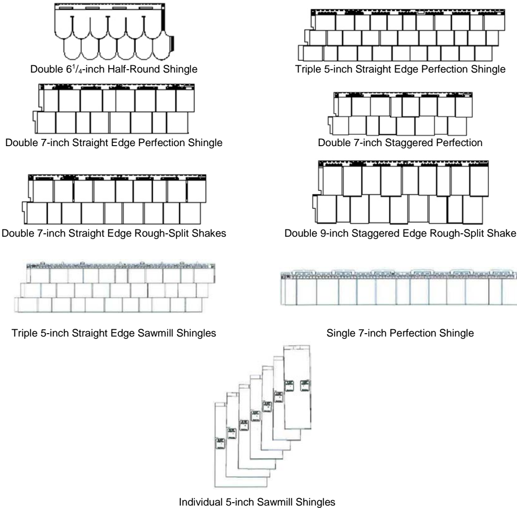
FIGURE 1—PRODUCT PROFILES
